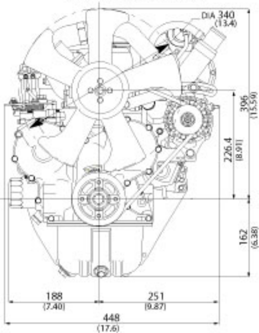
Vanguard 3/LC 31, 34 HP Turbo Diesel
