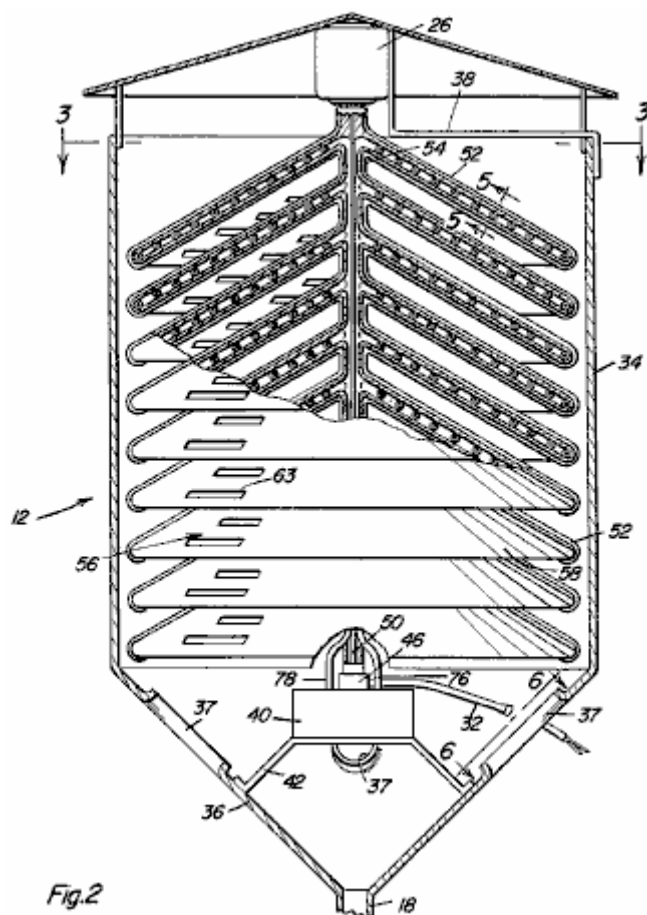
Fig.2 is a partial sectional view with parts shown in section of the apparatus.
