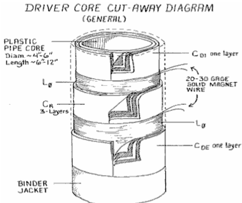
Fig.2 shows the "driver core" in a cutaway, perspective diagram. The PVC plastic "core" material can be a 6 inch (150 mm) diameter foot long (300 mm) piece of PVC pipe in this scaled-down model system. In this diagram, please note the inner and outer one-layer capacitor capacitors CDE and CDI . Also note that the middle capacitor
