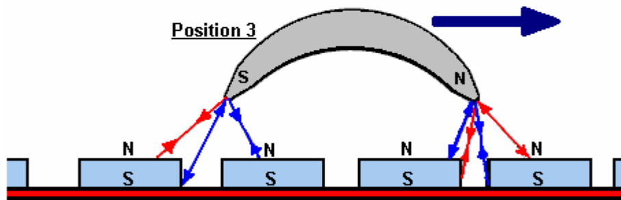
SIDE VIEWS
