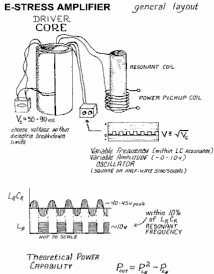
Fig.1 shows the general layout of the entire E-Stress Power System. This diagram illustrates the driver core and the variable frequency oscillator which determines the tank circuit resonance. Fig.1 also shows the DC power source of around 50 to 90 volts, which initially charges the "core" capacitor CDI / CDE . Also shown in this diagram is the resonant coil and power output or "pickup" coil.
