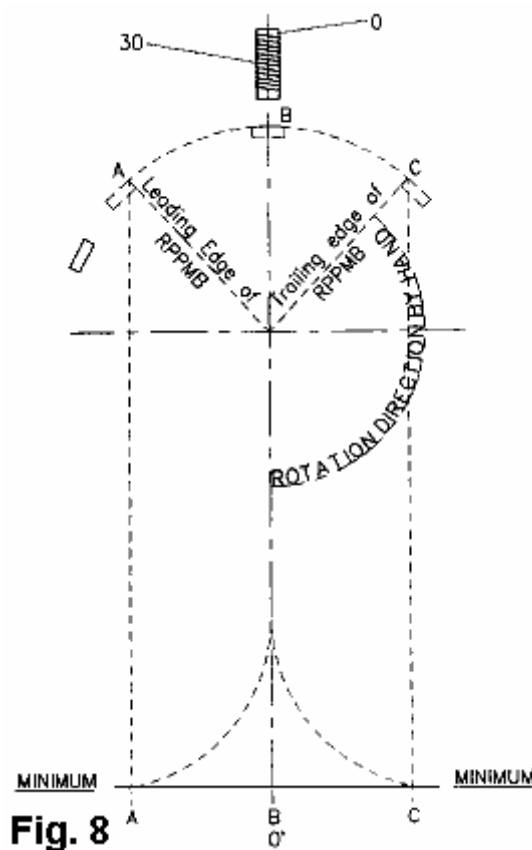
Fig.8 shows a schematic diagram of variation of natural magnetic attraction versus angular displacement of a rotor having a single permanent magnet and a stator having a single energising coil, in accordance with a second embodiment of the present invention;
