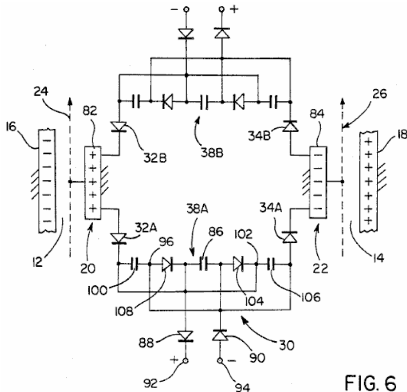
Fig.6 is an electrical circuit diagram of the output circuit of the generator shown in Fig.2, in accordance with one embodiment.
