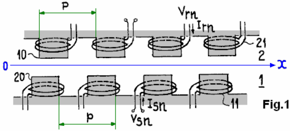
Fig.1 shows diagrammatically, a machine structure to which the invention is applied, in which the stator 1 and the rotor 2 comprise poles aligned in the direction o \rightarrow x along which the rotor movement occurs. These poles are marked as 10 and 20 and are repeated with the same horizontal spacing or pitch p in both the rotor and the stator. References 11 and 21 are the inductive windings through which the coupling occurs between a pole of the rotor and a pole of the stator when they align in the course of their movement.
