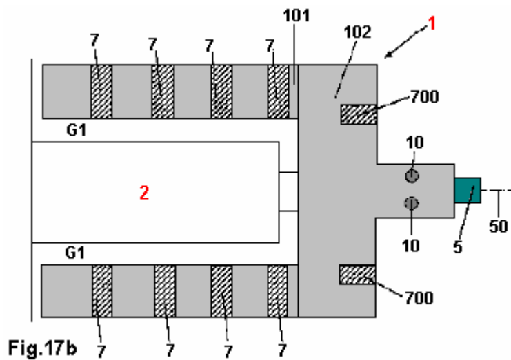
Fig.17b is a schematic view of one rotor drum and part of the inner stator 2 , where the view is perpendicular to the shaft axis 50 . The rotor 1 is clamped to the shaft 5 by the screws 10 and held rigidly in position. The shaft 5 passes through a ball bearing inset into the inner stator 2 and so can rotate freely relative to the inner stator. The rotor has two drum, or bell-shaped, sections which surround the inner stator. The rotor 1 has a hollow cylindrical section 101 , which extends away from the top surface 102 . Since the inner stator is fixed and prevented from rotation by it's anchoring device (component 4 in Fig.1 ), the rotor spins the hollow cylinder 101 around it. The hollow cylinder 101 of rotor 1 is separated from the inner stator 2 by an annular air gap G1 . The hollow cylinder 101 of rotor 1 has magnets 7 sunk into holes in it. The top surface 102 of the rotor 1 also has holes in it and these are used to install the magnets 700 in it.
