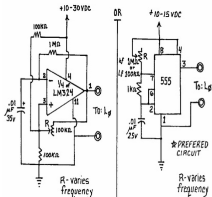
VARIABLE FREQUENCY OSCILLATORS
