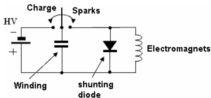
Fig. 8(A) Illustration of the idea of "zero resonance frequency" or the current accumulation..
