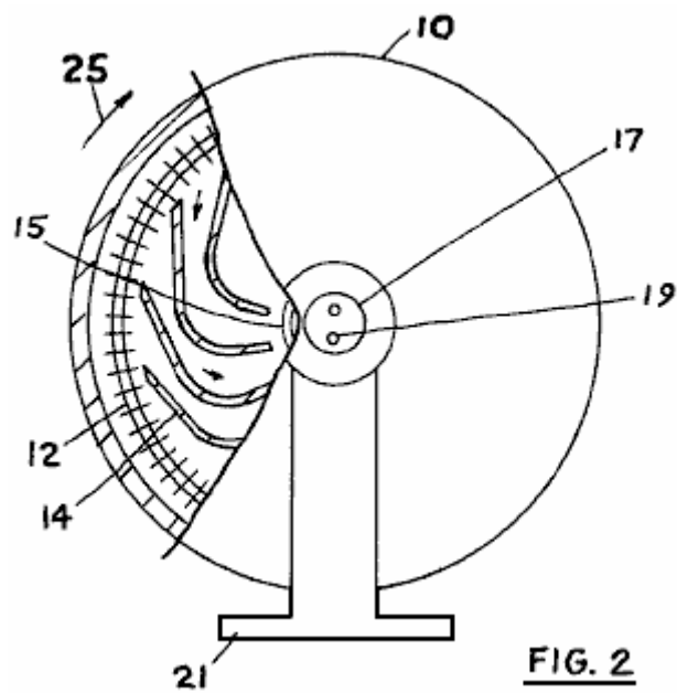
Fig.2 is an end view of a closed type rotor.
