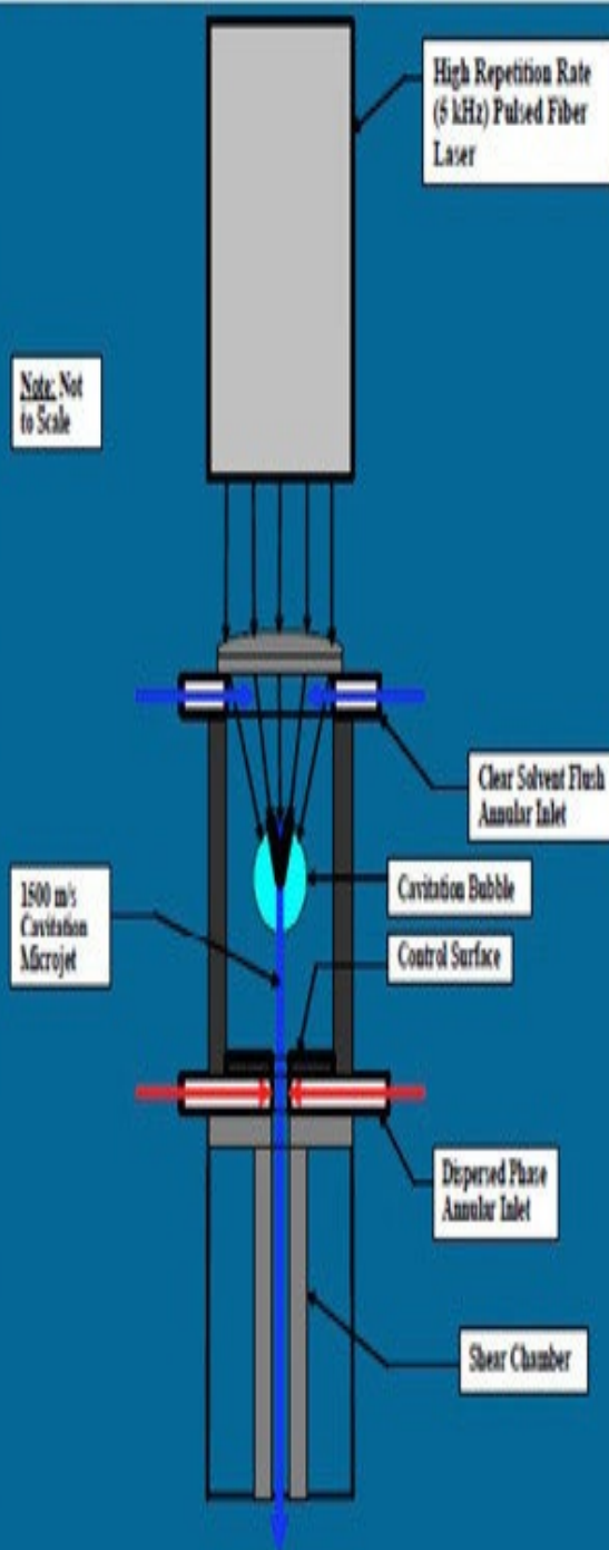
High Shear Cavitation Reentrant Jet Dispersion Module Schematic
